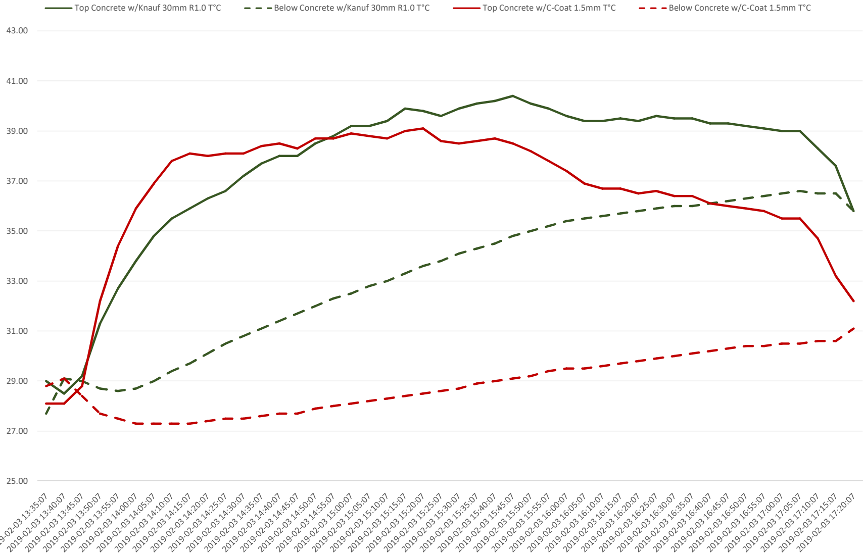
Summary Concrete Slab w/Knauf 30mm R1.0 vs. Slab with C-COAT 1.5mm on top 03.02.2019
